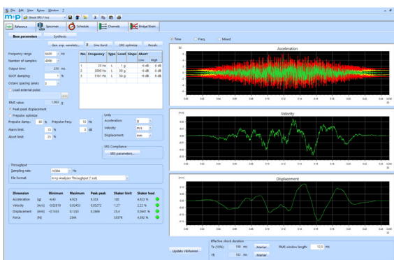
Setting up an SRS test
