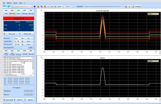
Classical shock testing
